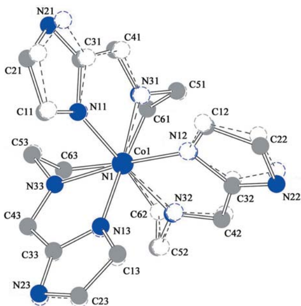
Figure 2 A least-squares fit between one cation and its 120° rotated image, showing the noncrystallographic pseudo- \text{C}_3 symmetry, viewed down the pseudo- \text{C}_3 axis.
